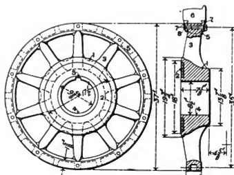
Figs. 4591-4592. Cast-Steel Driving Wheel Center for New York Central Electric Locomotive.
